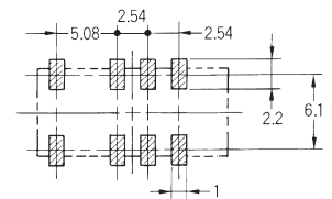
Footprint (Top View)
