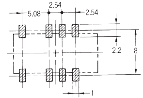
Footprint (Top View)
