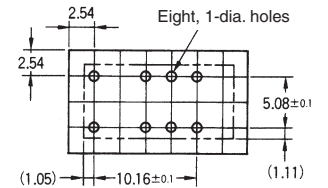
Footprint (Bottom View)
